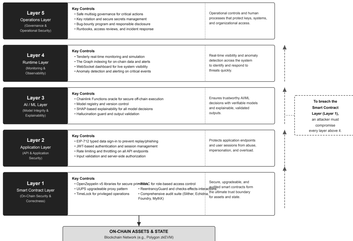
Figure 3.31: Five-layer defense-in-depth security architecture
